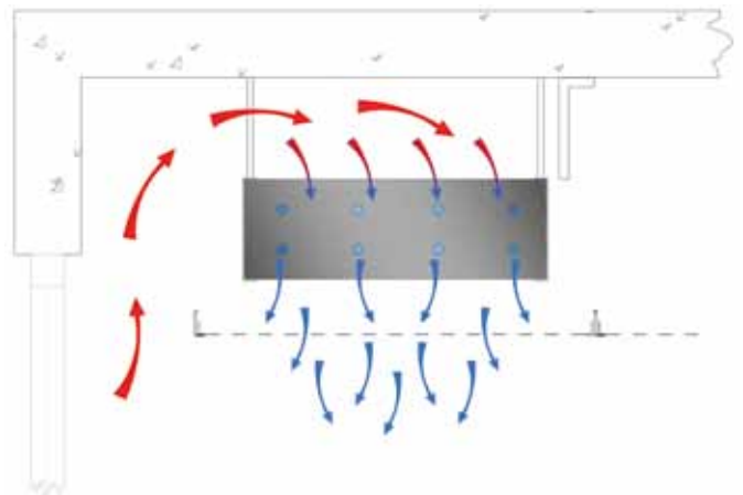
Figure 6: Perimeter passive chilled beam
