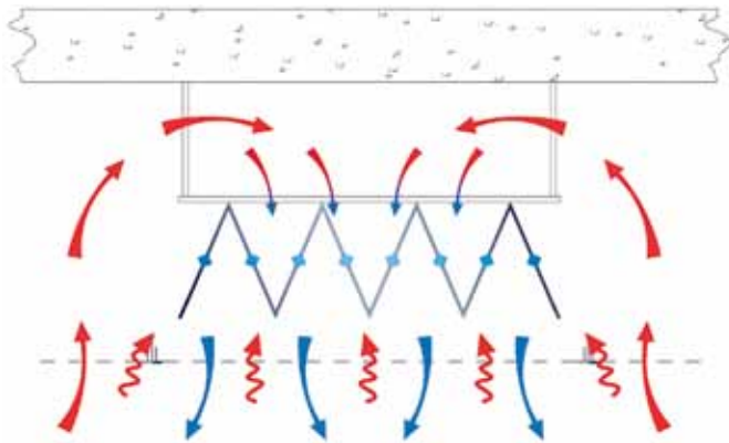
Figure 8: Radiant/convective beam above perforated ceiling
